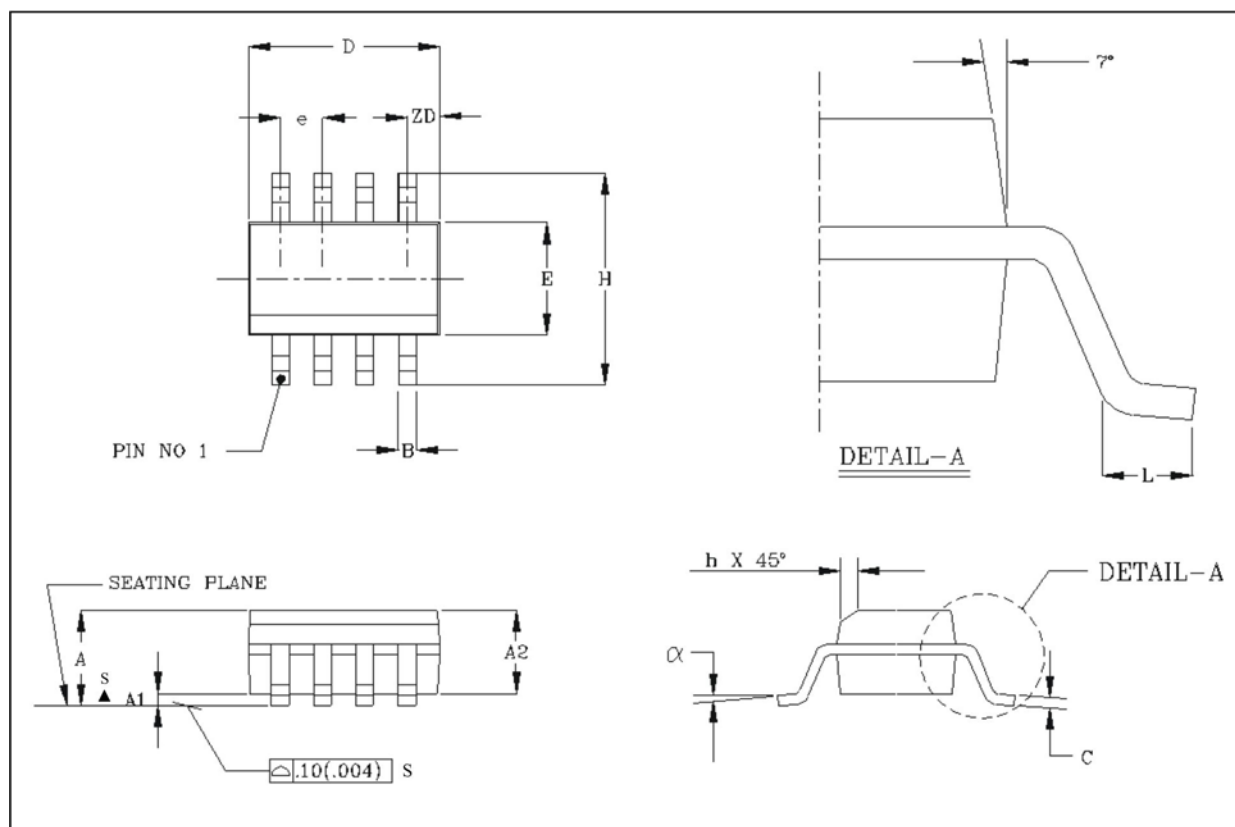
Figure 19: SOIC8 Drawing
