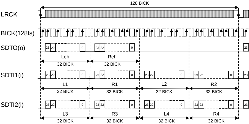
Figure 12. Mode 11 Timing
