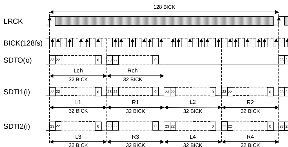
Figure 11. Mode 10 Timing
