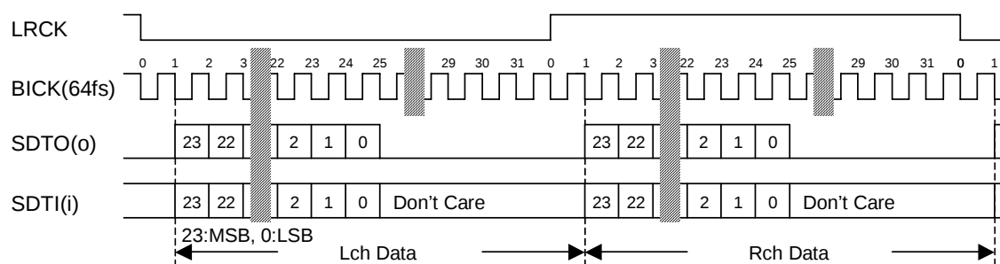
Figure 4. Mode 3 Timing
