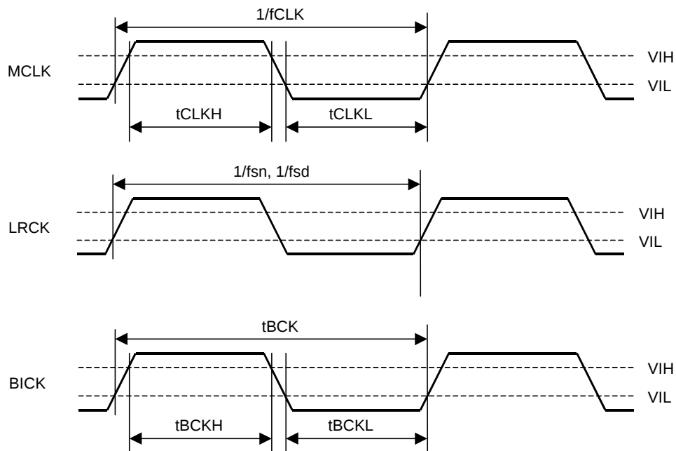
Clock Timing (TDM= "0")
