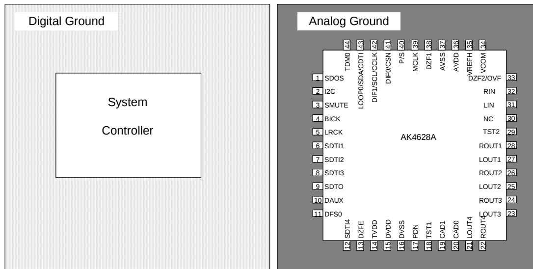
Figure 26. Ground Layout
