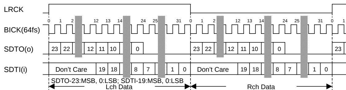
Figure 1. Mode 0 Timing
