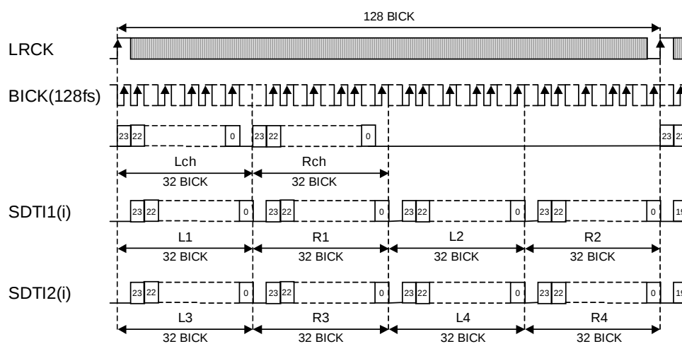
Figure 10. Mode 9 Timing
