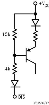
FIGURE 5. Equivalent of \overline{\text{DIS}} input
