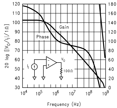
Open-Loop Transimpedance Gain, Z(s)
