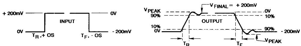
OVERSHOOT, RISE &amp; FALL TIME WAVEFORMS
