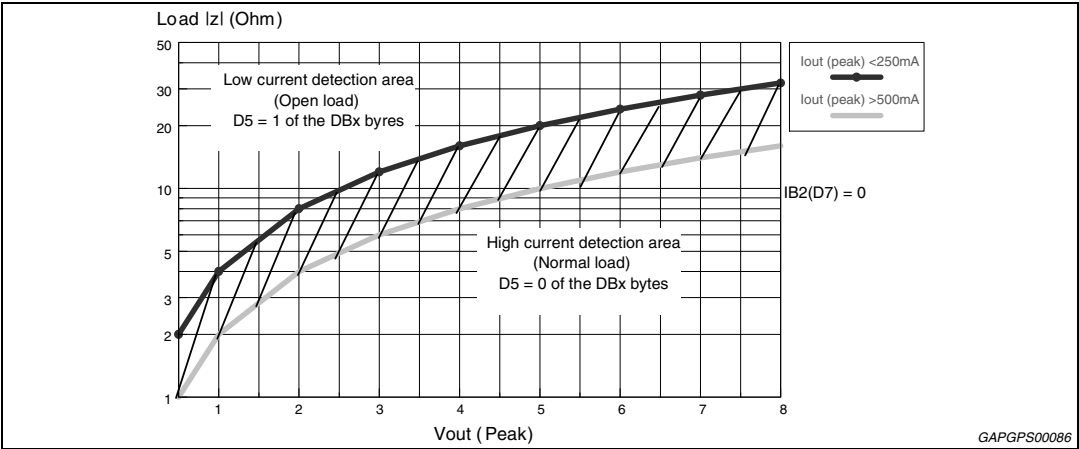
Figure 30. Current detection high: load impedance |Z| vs. output peak voltage
