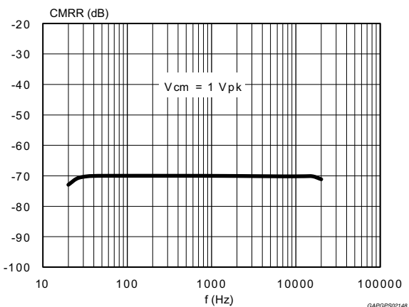
Figure 20. Input CMRR vs. frequency
