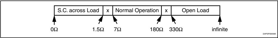
Figure 27. Load detection threshold - low gain setting
