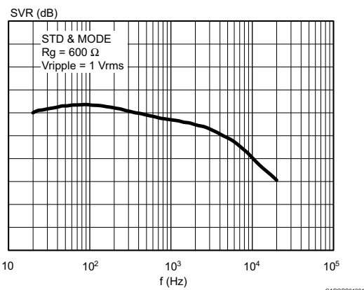
Figure 15. Supply voltage rejection vs. frequency
