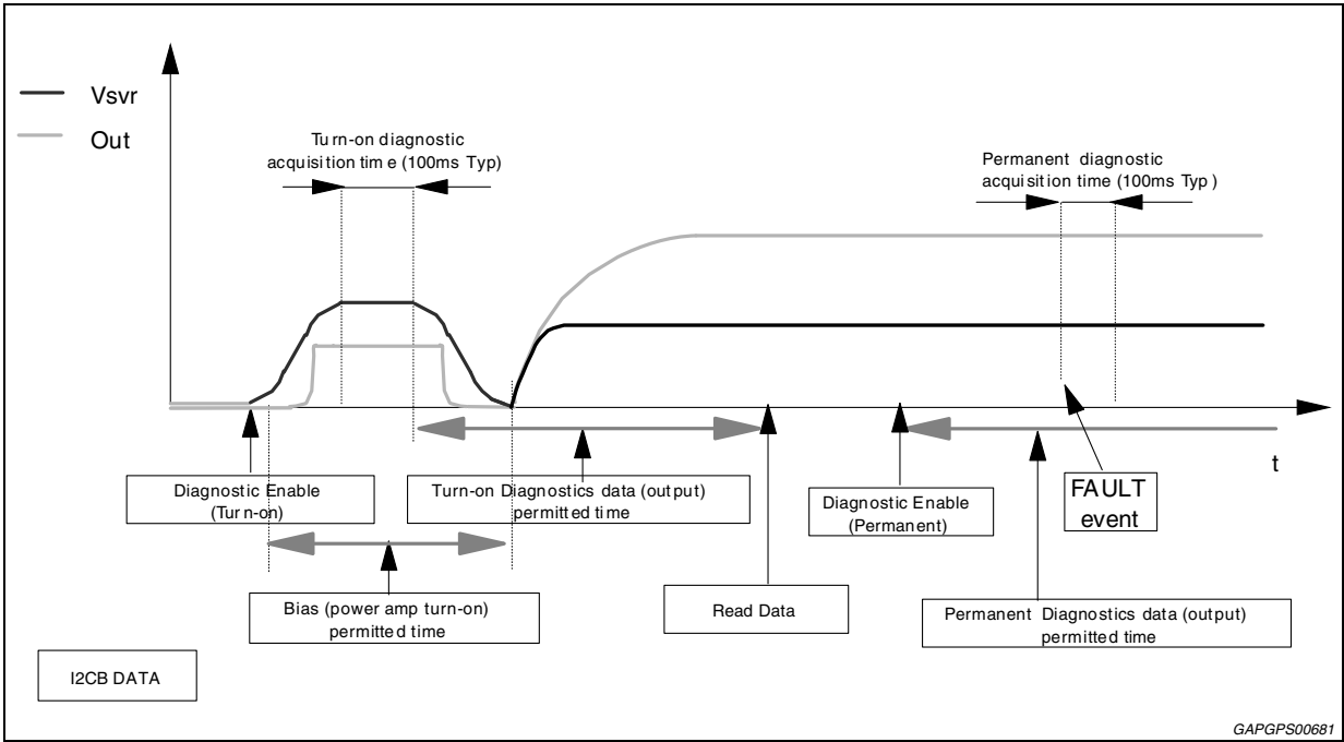
Figure 24. SVR and output pin behavior (Case 2: with turn-on diagnostic)
