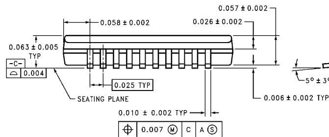
20-Lead Quarter Size Outline Package (QSOP), JEDEC MO-137, 0.150" Wide Package Number MQA20
