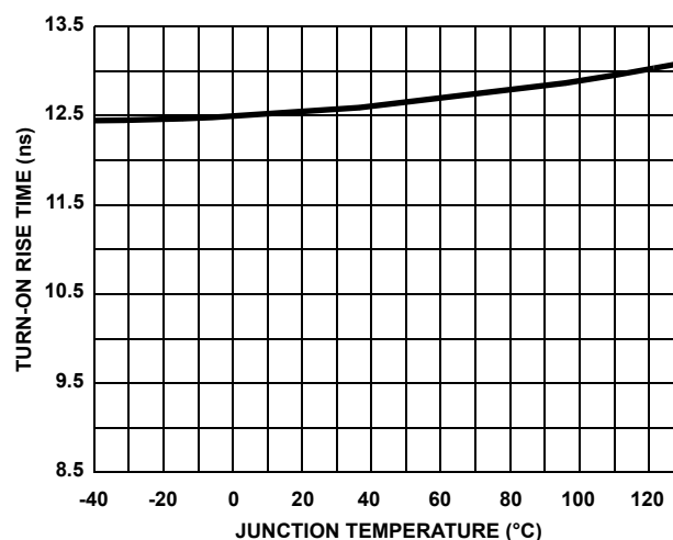
FIGURE 23. GATE DRIVE RISE TIME t_r vs TEMPERATURE
