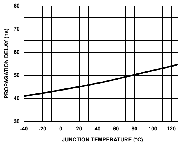
FIGURE 15. LOWER DISABLE TURN-OFF PROPAGATION DELAY t_{DISLOW} vs TEMPERATURE
