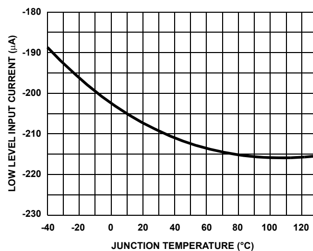
FIGURE 11. HEN LOW LEVEL INPUT CURRENT I_{IL} vs TEMPERATURE
