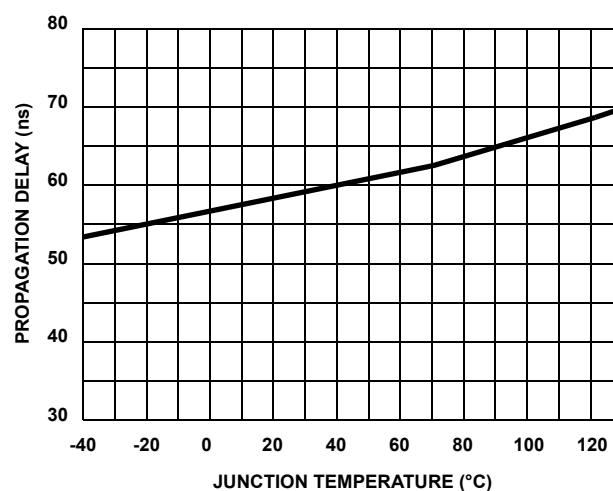
FIGURE 13. UPPER DISABLE TURN-OFF PROPAGATION DELAY t_{DISHIGH} vs TEMPERATURE
