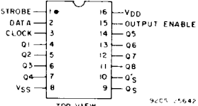
Fig. 1 — Terminal assignment.
