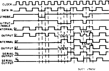
Fig. 3 — Timing diagram.
