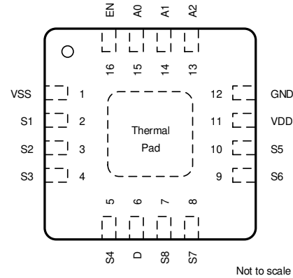
Figure 6-2. TMUX7208: RUM Package 16-Pin WQFN Top View
