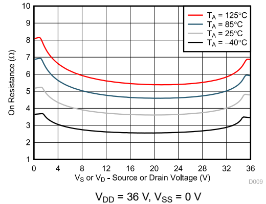
Figure 7-8. On-Resistance vs Temperature
