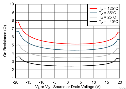
Figure 7-6. On-Resistance vs Temperature V_{DD} = 20\text{ V}, V_{SS} = -20\text{ V}
