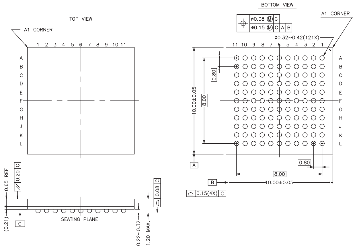
Figure 21-1. AT91FR40162S Package
