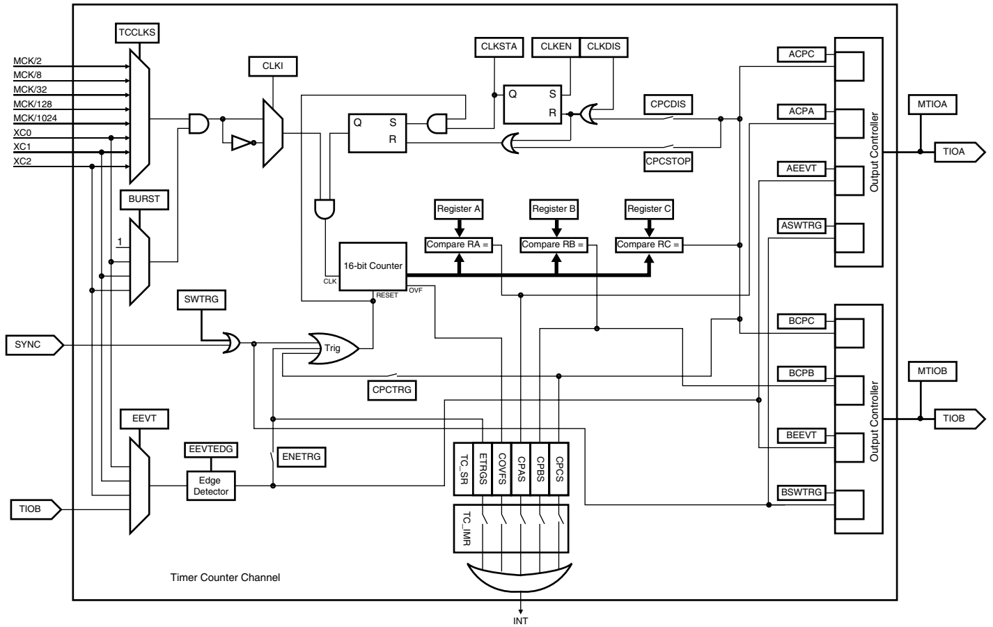
Figure 18-5. Waveform Mode
