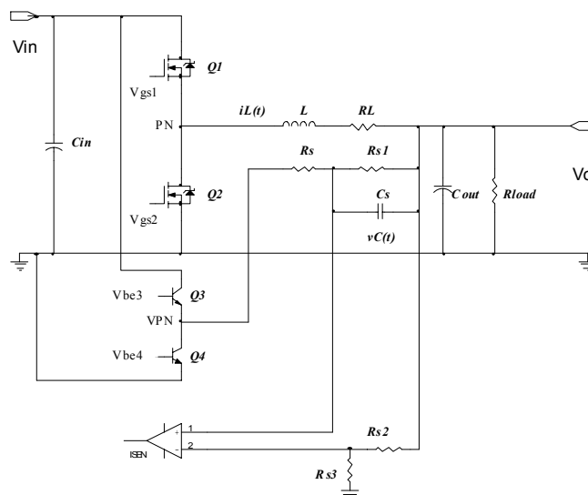
Figure 16. Scaling the equivalent current limit.
