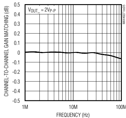
CHANNEL-TO-CHANNEL GAIN MATCHING vs. FREQUENCY
