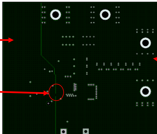
Fig. 26c. IR3831 layout considerations – Mid Layer 1
