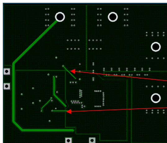
Fig. 26d. IR3831 layout considerations – Mid Layer 2
