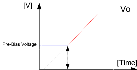
Fig. 4. Pre-Bias startup
