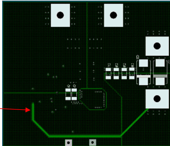
Fig. 26b. IR3831 layout considerations – Bottom Layer
