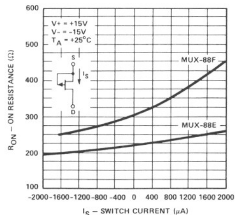
R ON vs SWITCH CURRENT (I S )
