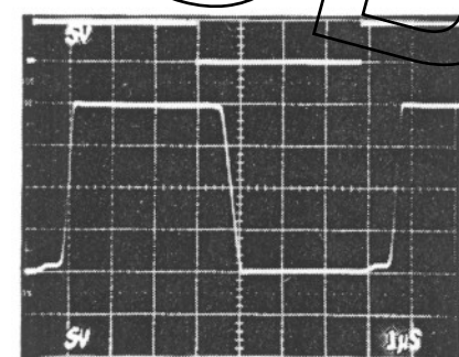
LARGE-SIGNAL SWITCHING
