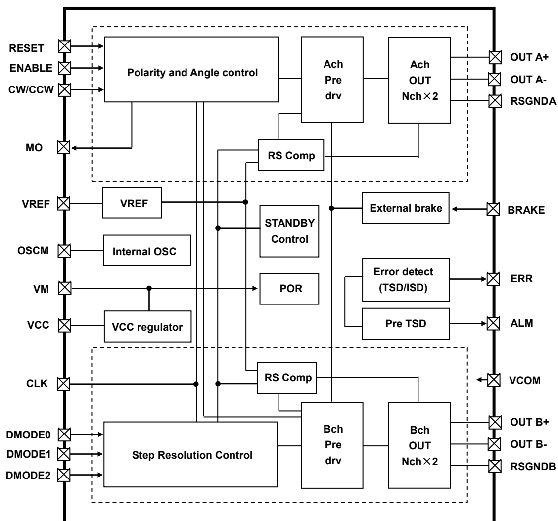
TB67S149 block diagram
