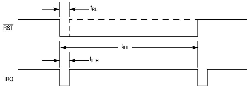
Figure 19-3. \overline{RST} and \overline{IRQ} Timing
