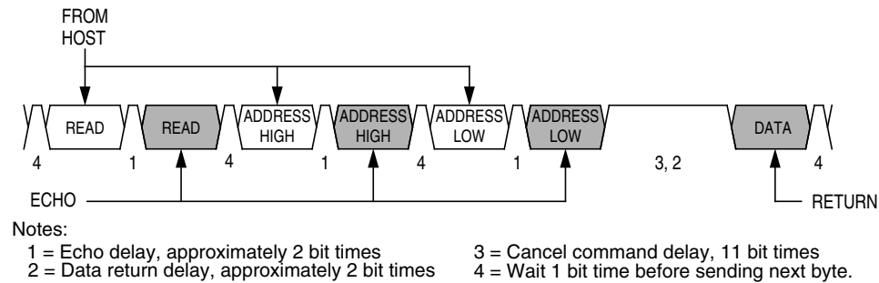
Figure 18-15. Read Transaction
