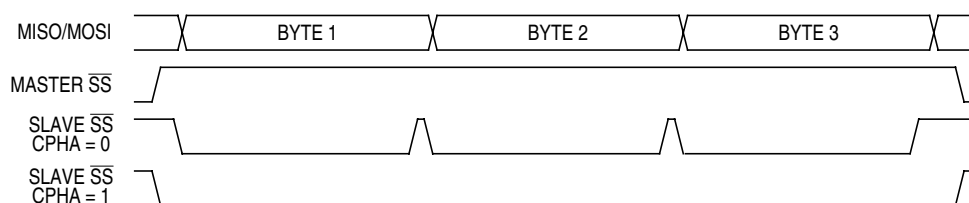
Figure 15-5. CPHA/\overline{SS} Timing
