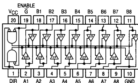
SN54/74LS641 SN54/74LS645
