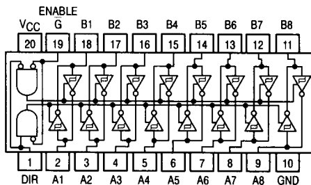
SN54/74LS640 SN54/74LS642
