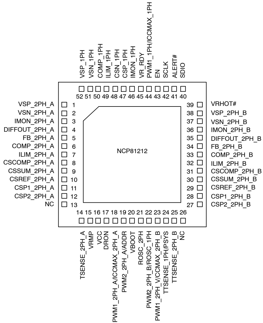
Figure 2. Pinout Diagram
