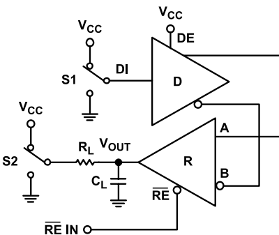
Figure 43. Receiver Enable/Disable from Shutdown
