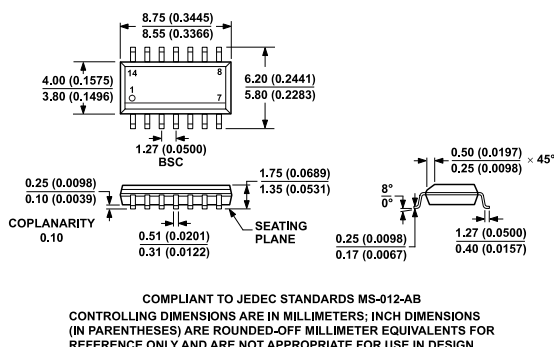
Figure 54. 14-Lead Standard Small Outline Package [SOIC_N] Narrow Body (R-14) Dimensions shown in millimeters and (inches)
