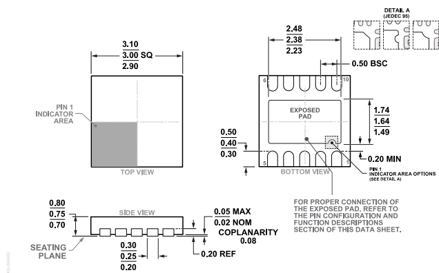
Figure 53. 10-Lead Lead Frame Chip Scale Package [LFCSP] 3 mm x 3 mm Body and 0.75 mm Package Height (CP-10-9) Dimensions shown in millimeters
