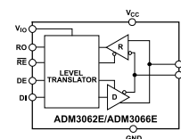
Figure 3. ADM3062E/ADM3066E Functional Block Diagram
