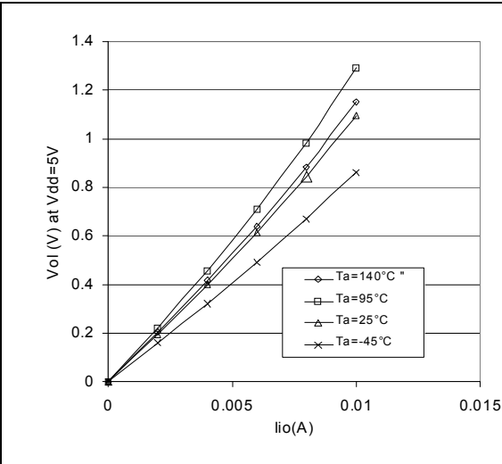
Figure 81. Typical V_{OL} at V_{DD} = 5V (standard)
