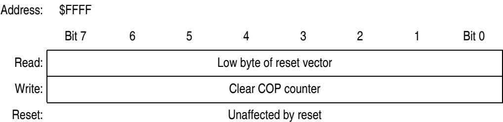
Figure 15-3. COP Control Register (COPCTL)
