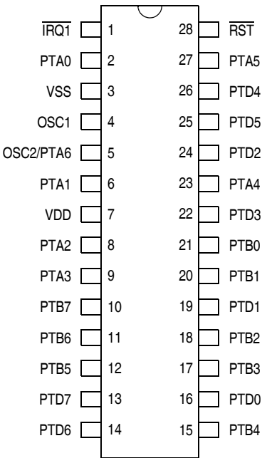
28-PIN ASSIGNMENT MC68H(R)C08JL3
