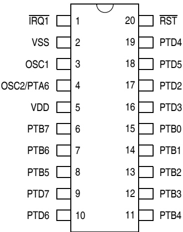
20-PIN ASSIGNMENT MC68H(R)C08JK3/JK1
