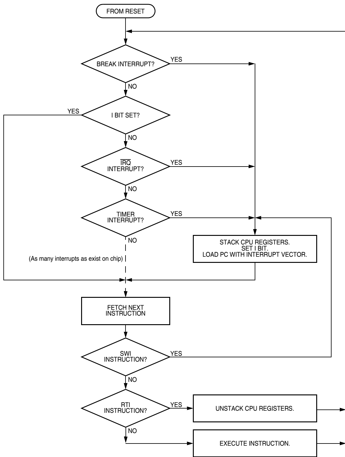
Figure 7-8. Interrupt Processing
