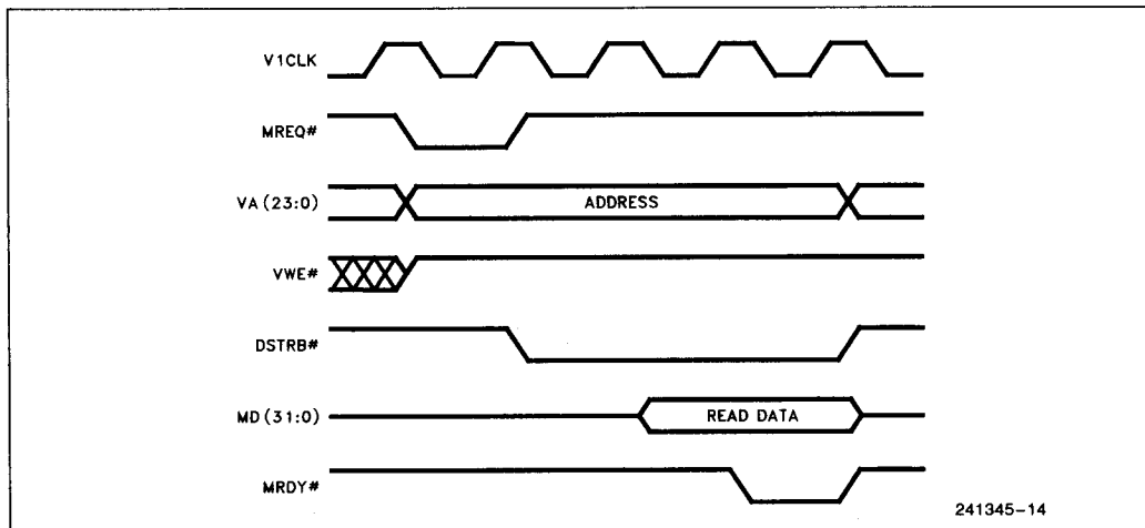
Figure 3-8. Register Read Cycle
