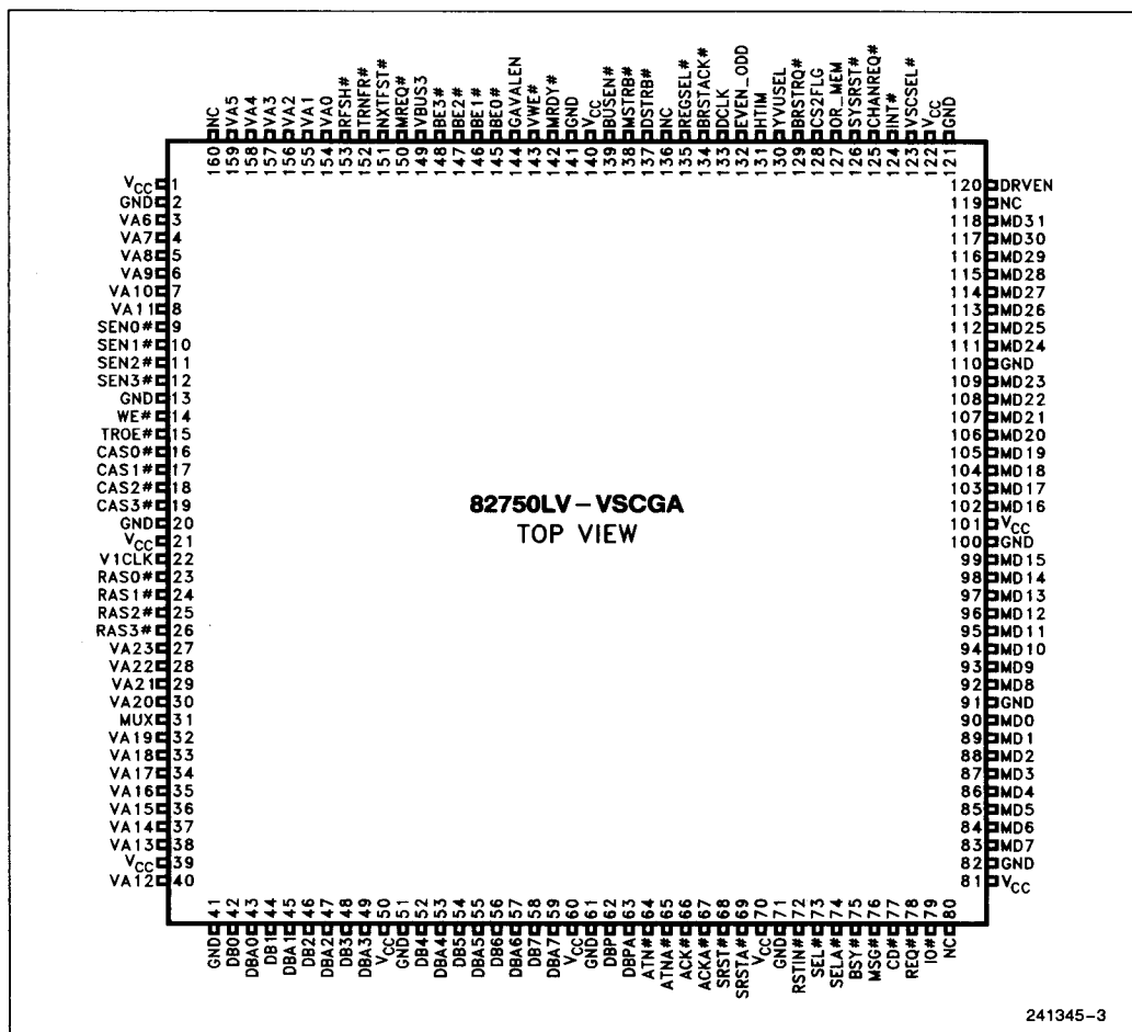
Figure 1-1. 82750LV Pinout
