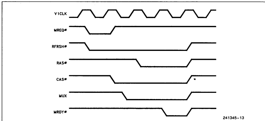
Figure 3-7. Refresh Cycle
