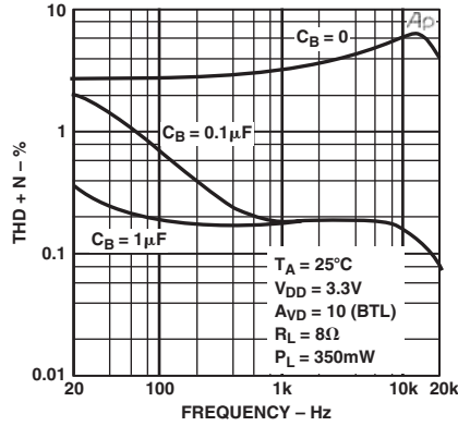
TPC 11. THD+N vs. Frequency
