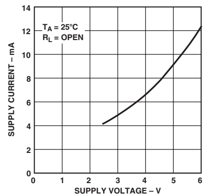
TPC 30. Supply Current vs. Supply Voltage
