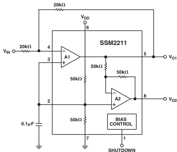
Figure 1. Simplified Schematic
