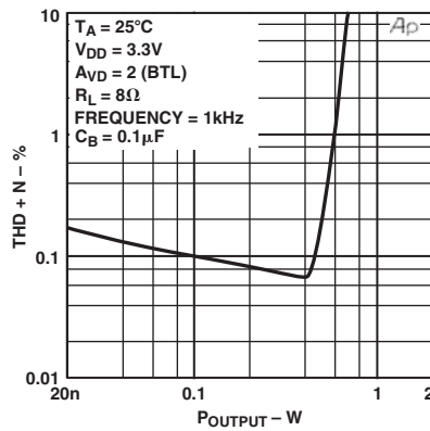
TPC 14. THD+N vs. P_{\text{OUTPUT}}
