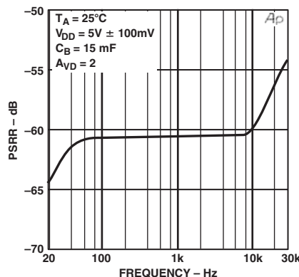
TPC 37. PSRR vs. Frequency
