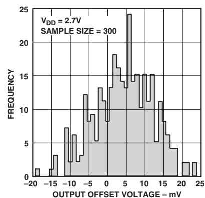
TPC 33. Output Offset Voltage Distribution
