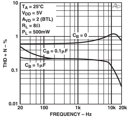
TPC 1. THD+N vs. Frequency
