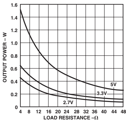
TPC 31. P_{OUT} vs. Load Resistance
