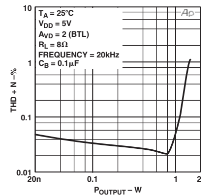
TPC 9. THD+N vs. P_{OUTPUT}
