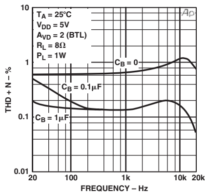
TPC 4. THD+N vs. Frequency
