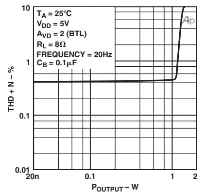
TPC 7. THD+N vs. P_{OUTPUT}
