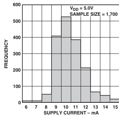
TPC 36. Supply Current Distribution
