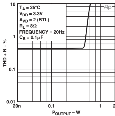
TPC 13. THD+N vs. P_{\text{OUTPUT}}
