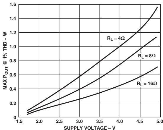
Figure 6. Maximum Output Power vs. V_{SY}
