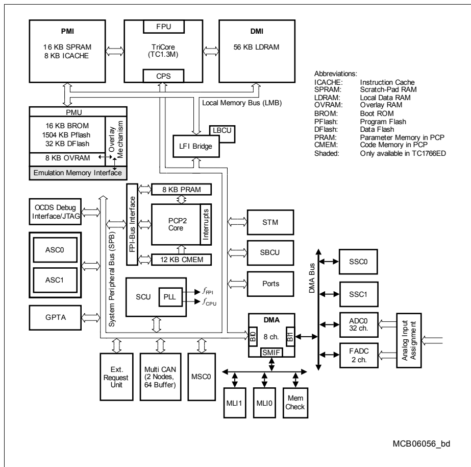
Figure 1 TC1766 Block Diagram
