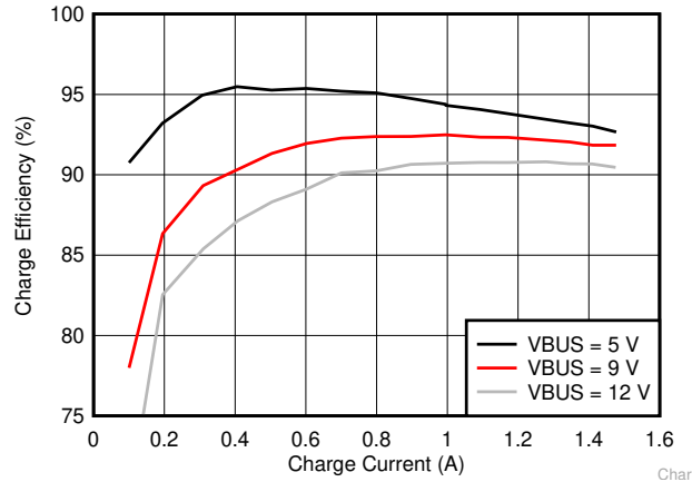
Figure 8-1. Charge Efficiency
