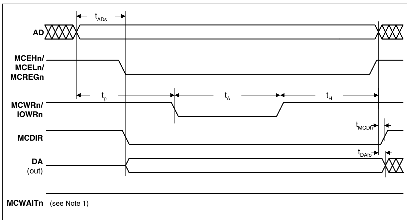
Figure 18. PCMCIA Write Cycle Timing Measurement
