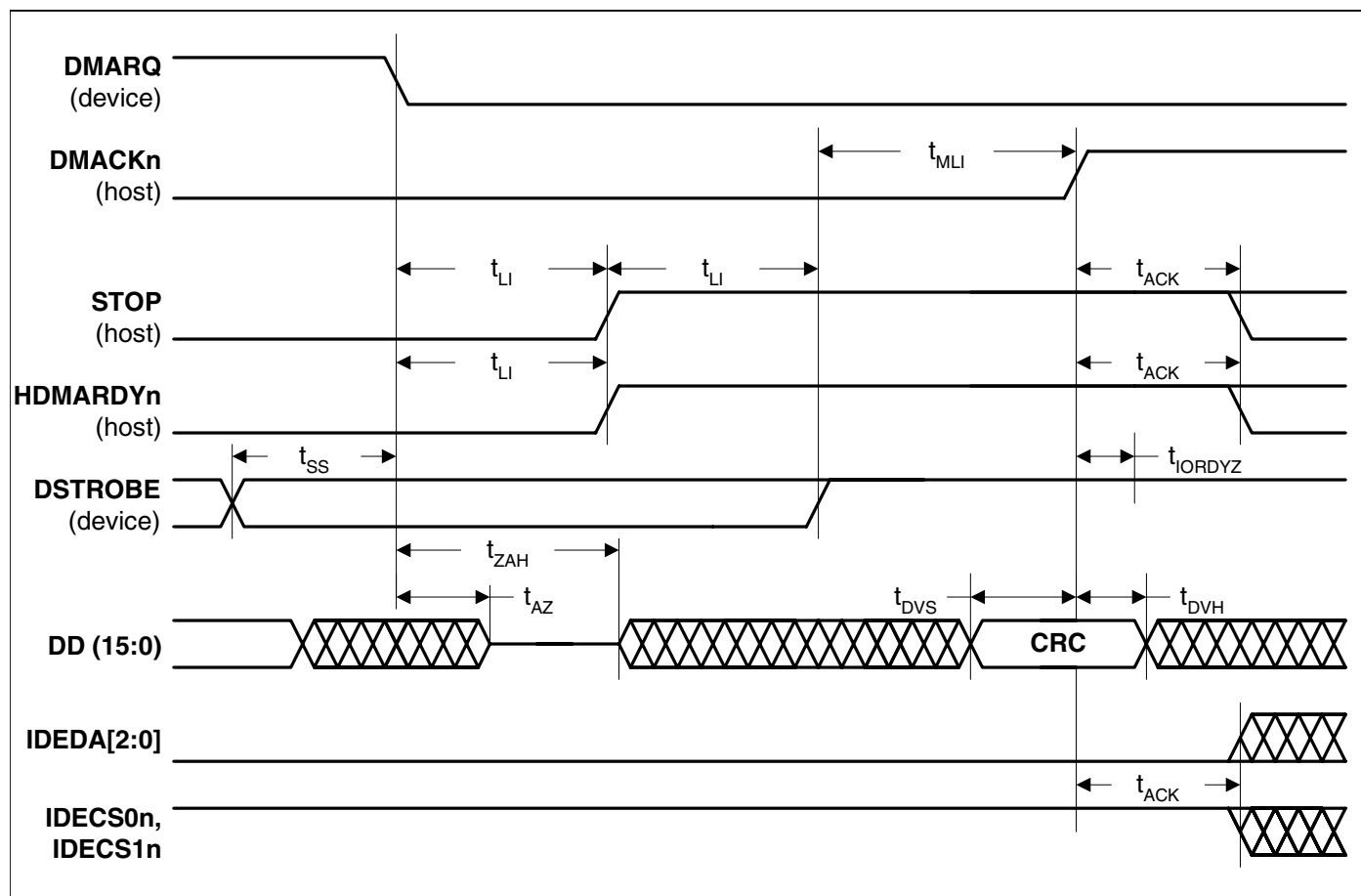
Figure 24. Device Terminating an Ultra DMA data-in Burst
