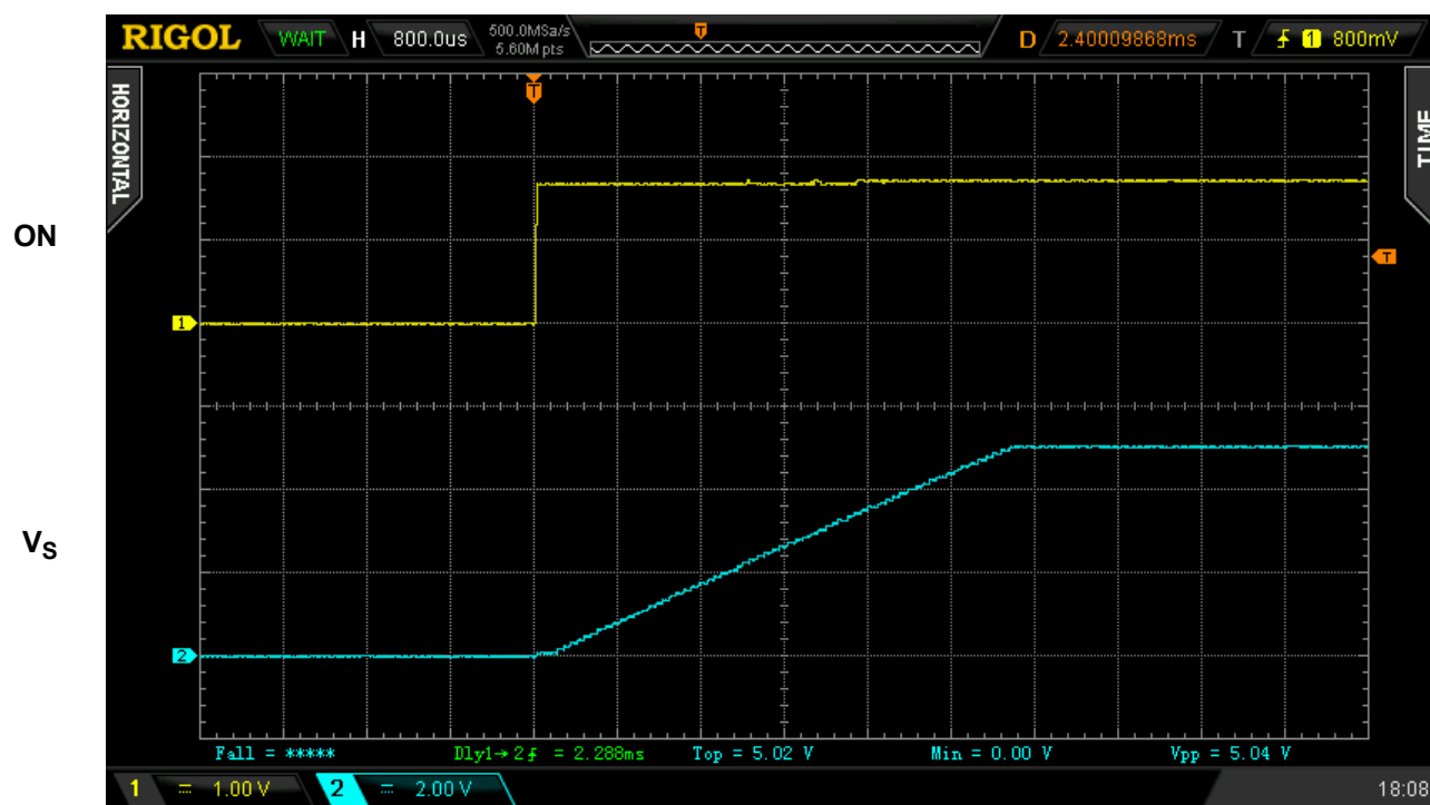
Figure 2. Typical Turn ON operation waveform for V_{DD} = V_D = 5\text{ V} , C_{SLEW} = 12\text{ nF} , C_{LOAD} = 10\text{ }\mu\text{F} , R_{LOAD} = 20\text{ }\Omega
