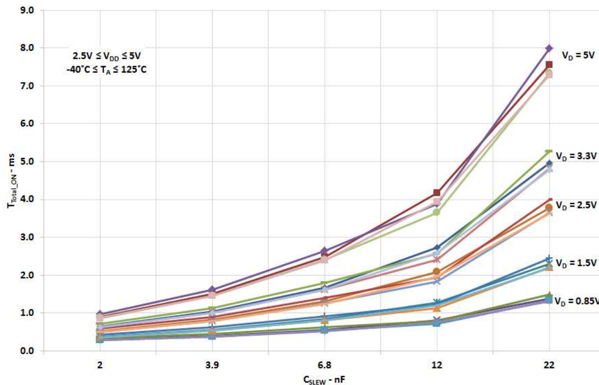
T_{Total\_ON} vs. C_{SLEW} , V_D , V_{DD} , and Temperature
