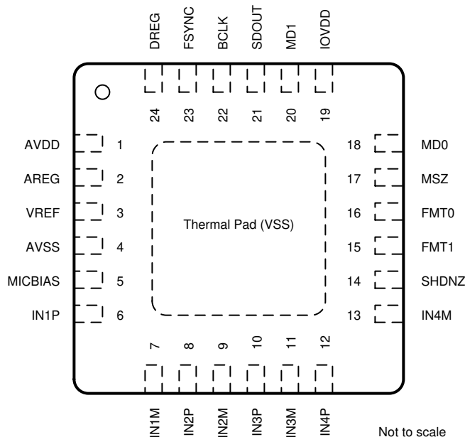
Pin Functions
