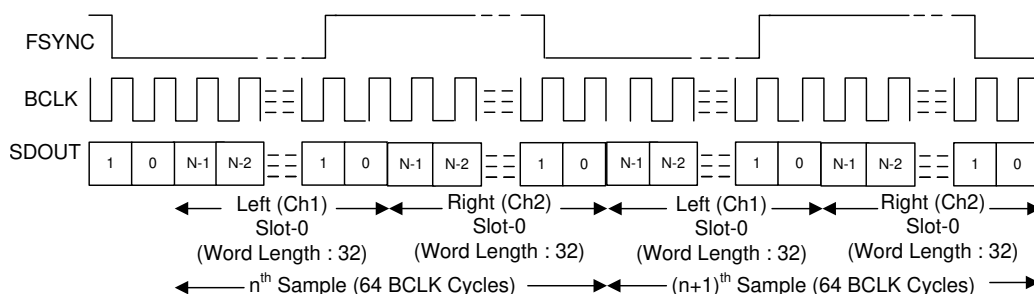
Figure 19. I²S Protocol Timing In Master Mode
