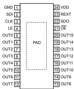
LP Package
