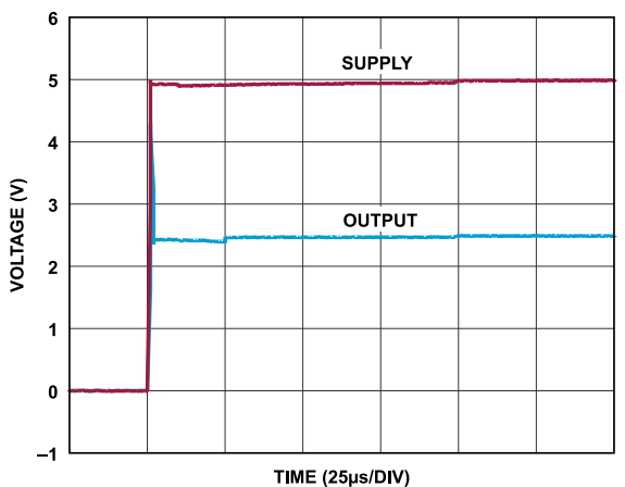
Figure 34. Start-Up Response
