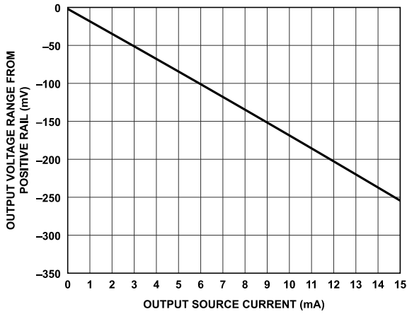
Figure 32. Output Voltage Range from Positive Rail vs. Output Source Current
