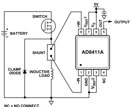
Figure 61. High-Side Switch
