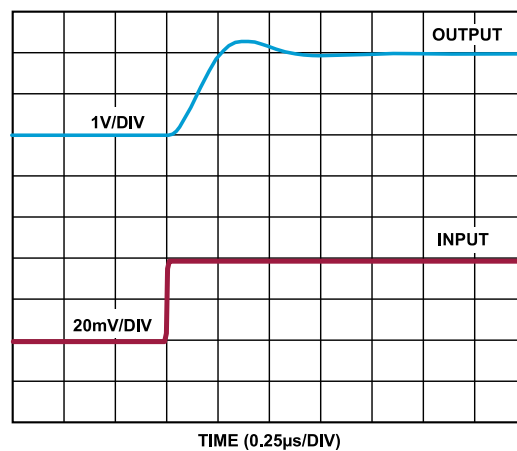
Figure 20. Rise Time, V_S = 5\text{ V}
