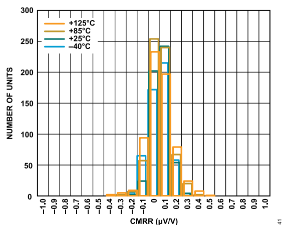
Figure 43. CMRR Distribution
