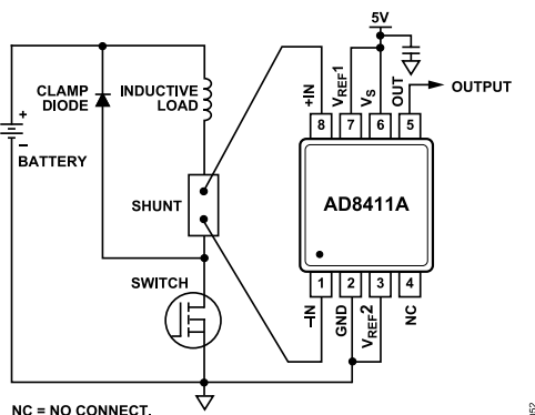
Figure 60. Low-Side Switch
