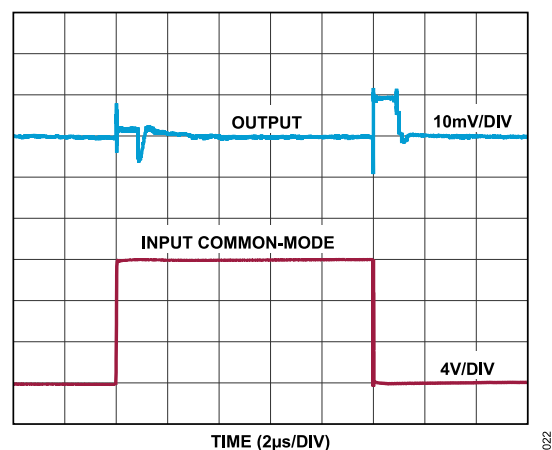
Figure 9. Input Common-Mode Step Response (0 V to 12 V), V_S = 5 V, Inputs Shorted
