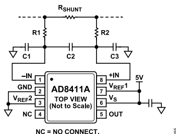
Figure 63. Input Filter
