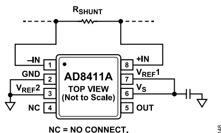
Figure 48. Shunt Resistor Layout
