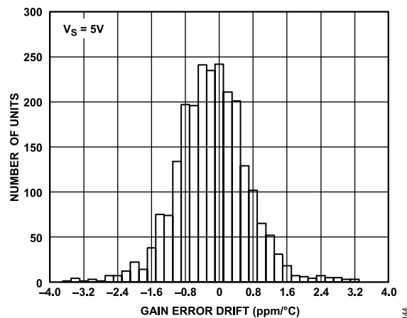
Figure 46. Gain Error Drift Distribution
