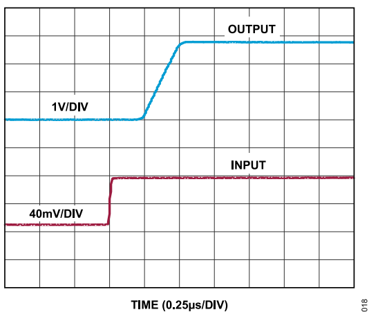
Figure 23. Differential Overload Recovery, Rising, V_S = 2.9\text{ V}
