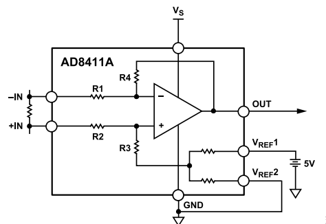
Figure 54. Split External Reference
