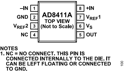
Figure 4. Pin Configuration
