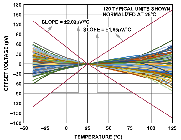
Figure 57. Bowtie Method
