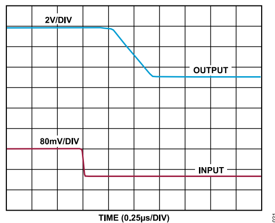
Figure 26. Differential Overload Recovery, Falling, V_S = 5\text{ V}
