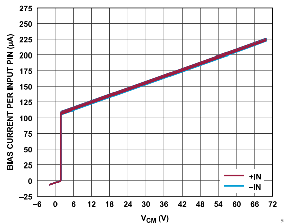
Figure 14. Bias Current Per Input Pin vs. V_{CM} , V_S = 5\text{ V}
