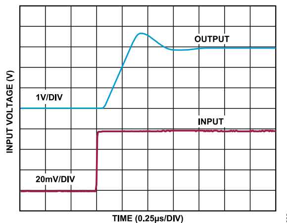
Figure 28. Large Signal Response, Rising, V_S = 5\text{ V}
