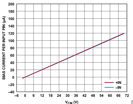
Figure 15. Bias Current Per Input Pin vs. V_{CM} , V_S = 0\text{ V} , R_L = 10\text{ k}\Omega
