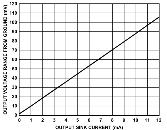
Figure 33. Output Voltage Range from Ground vs. Output Sink Current
