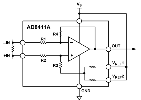
Figure 51. V_S Referenced Output
