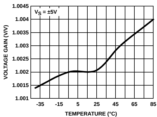
FIGURE 12. VOLTAGE GAIN vs TEMPERATURE
