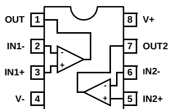
EL2244 (8-PIN SO, PDIP) TOP VIEW
