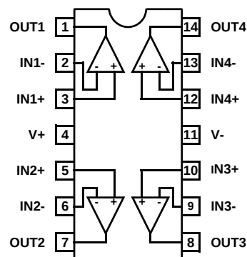
EL2444 [14-PIN SO (0.150"), PDIP] TOP VIEW
