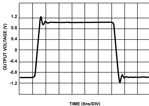
FIGURE 2. LARGE SIGNAL PULSE RESPONSE
