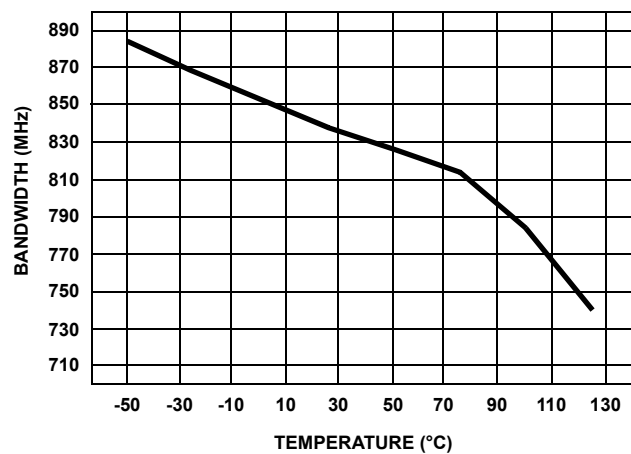
FIGURE 6. -3dB BANDWIDTH vs TEMPERATURE
