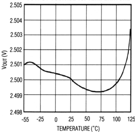
MAX873 OUTPUT VOLTAGE vs. TEMPERATURE
