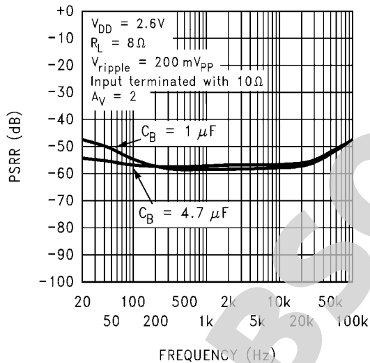
Power Supply Rejection Ratio (PSRR) @ V_{DD} = 2.6V
