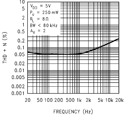
THD+N vs Frequency at V_{DD} = 5V , 8\Omega R_L , and PWR = 250mW
