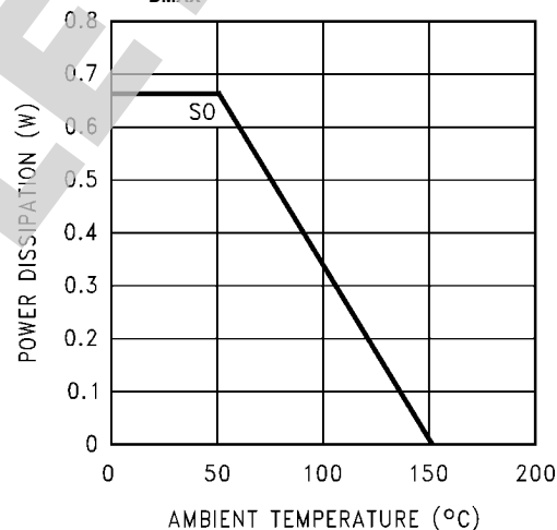
Power Derating - SOP P_{DMAX} = 670mW for 5V, 8Ω
