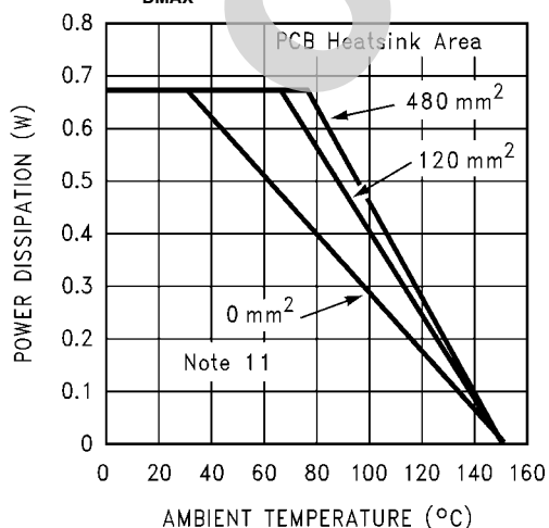
Power Derating - 9 Bump μSMD P_{DMAX} = 670mW for 5V, 8Ω
