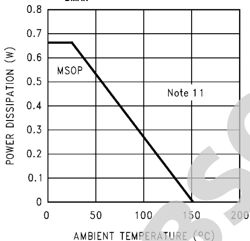
Power Derating - MSOP P_{DMAX} = 670mW for 5V, 8Ω
