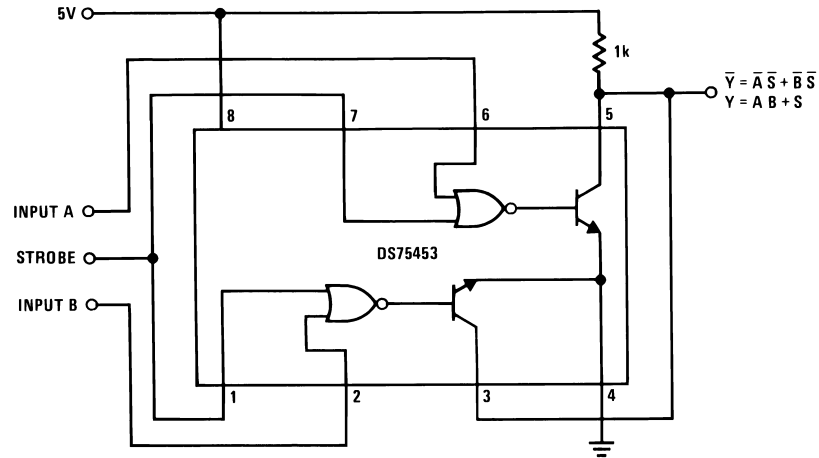
FIGURE 21. Logic Signal Comparator
