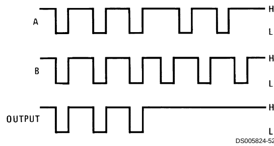
FIGURE 22. In-Phase Detector
