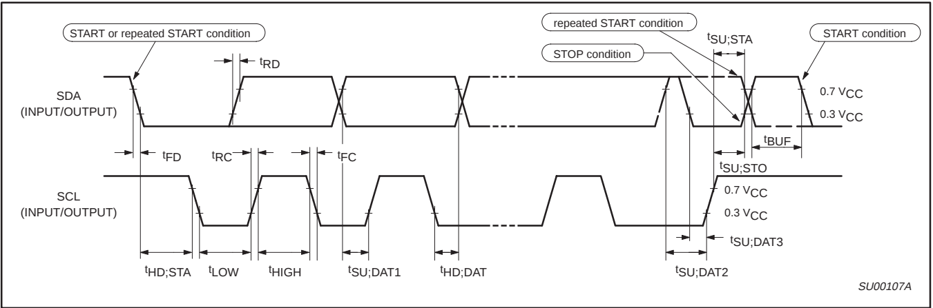
Figure 65. Timing SI01 (I²C) Interface
