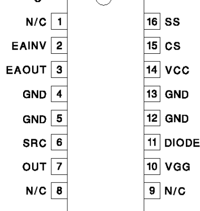
DIL-16, SOIC-16 (Top View) N or DP Packages
