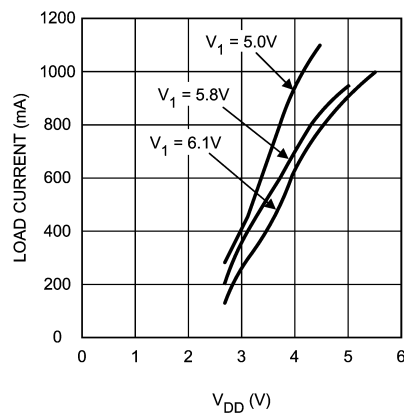
Load Current vs V_{DD}
