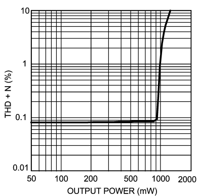
THD+N vs Output Power V_{DD} = 3V , A_V = 6dB , R_L = 8\Omega
