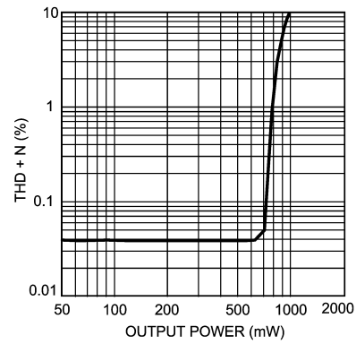
THD+N vs Output Power V_{DD} = 4.2V , A_V = 6dB , R_L = 16\Omega
