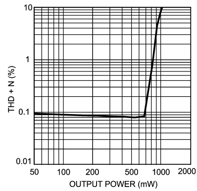
THD+N vs Output Power V_{DD} = 4.2V , A_V = 26dB , R_L = 16\Omega
