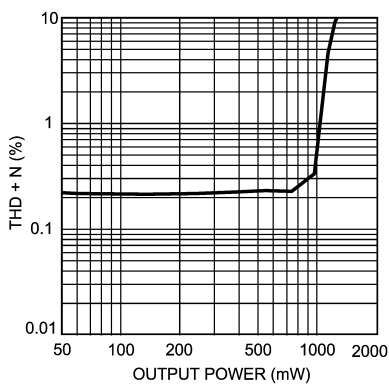
THD+N vs Output Power V_{DD} = 3V , A_V = 26dB , R_L = 8\Omega
