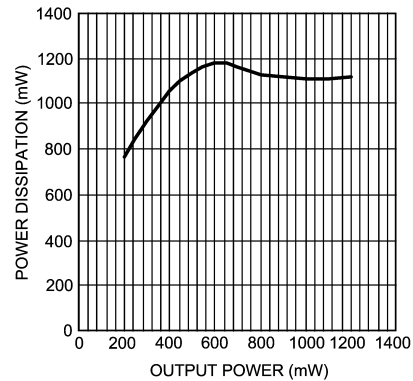
Power Dissipation vs Output Power V_{DD} = 3V , R_L = 8\Omega , f = 1kHz
