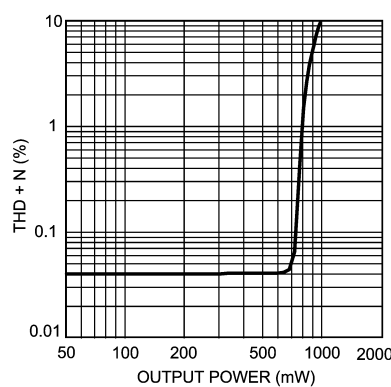
THD+N vs Output Power V_{DD} = 3V , A_V = 6dB , R_L = 16\Omega
