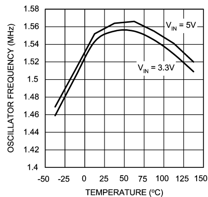
Oscillator Frequency vs Temperature - "X"
