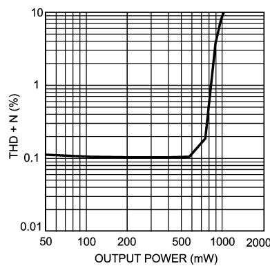
THD+N vs Output Power V_{DD} = 3V , A_V = 26dB , R_L = 16\Omega
