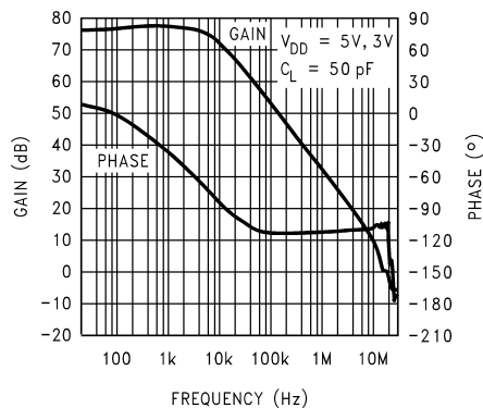
Amplifier Open Loop vs Frequency Response
