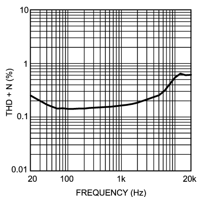
THD+N vs Frequency V_{DD} = 4.2V , A_V = 26dB , R_L = 8\Omega
