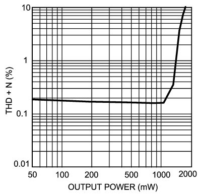
THD+N vs Output Power V_{DD} = 4.2V , A_V = 26dB , R_L = 8\Omega
