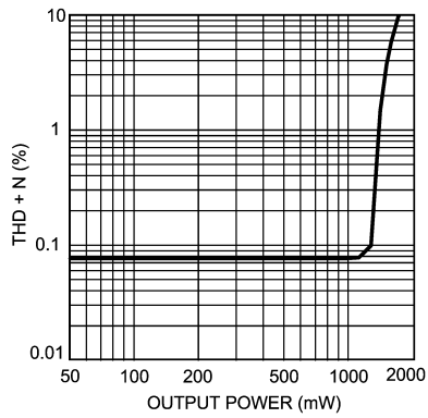
THD+N vs Output Power V_{DD} = 4.2V , A_V = 6dB , R_L = 8\Omega
