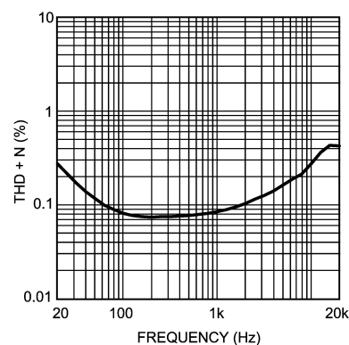
THD+N vs Frequency V_{DD} = 4.2V , A_V = 26dB , R_L = 16\Omega
