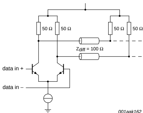
Fig 5. DC coupling
