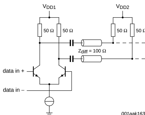
Fig 6. AC coupling
