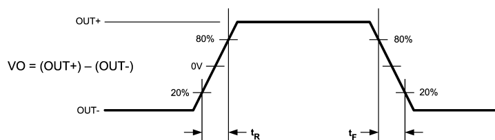
Figure 3. LPDS Output Transition Times
