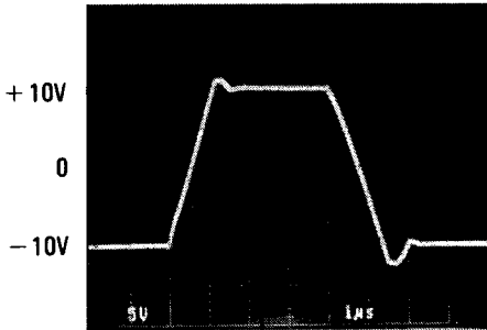
Large-Signal Pulse Response, A_V = +5
