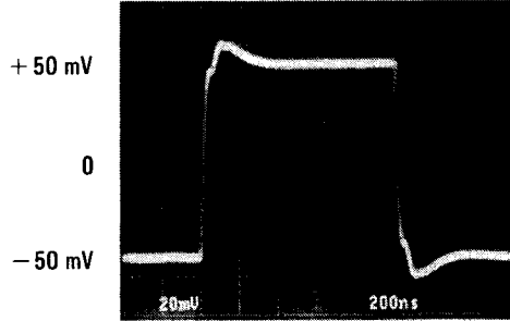
Small-Signal Pulse Response, A_V = +5
