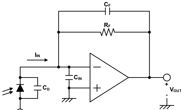
Figure1. Transimpedance amplifier
