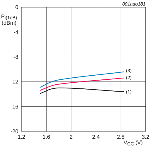
f = 1575 MHz. (1) T_{amb} = -40 °C (2) T_{amb} = +25 °C (3) T_{amb} = +85 °C
