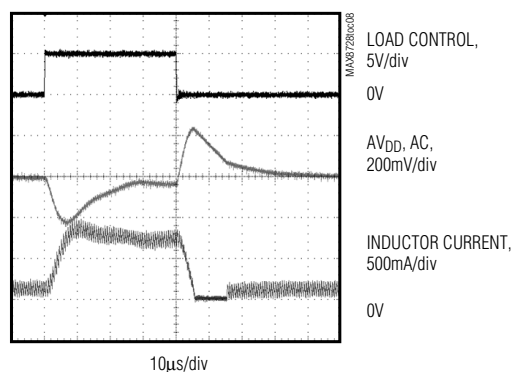
STEP-UP REGULATOR LOAD TRANSIENT RESPONSE (100mA TO 600mA)
