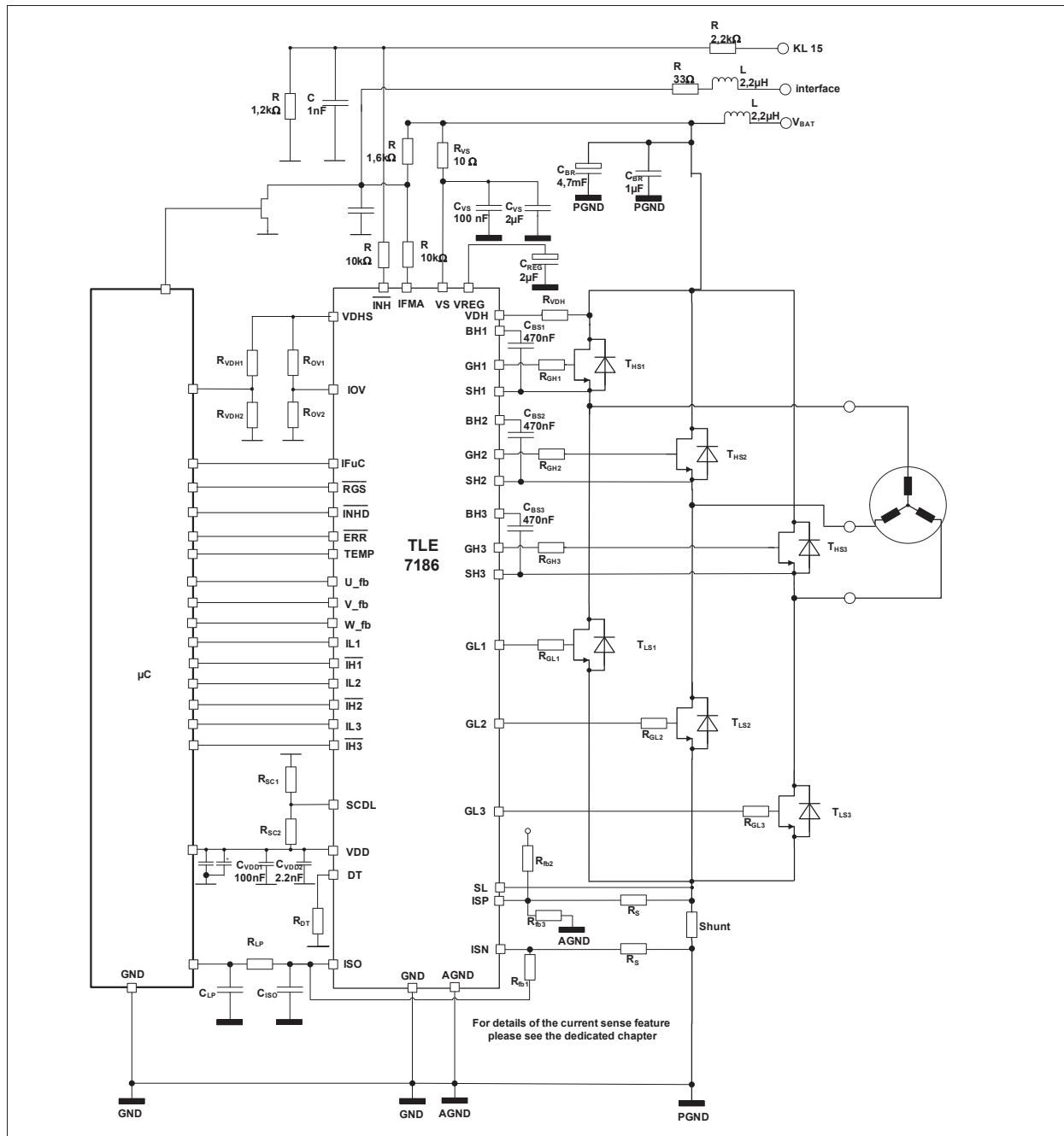
Figure 15 Application Circuit TLE7186F
