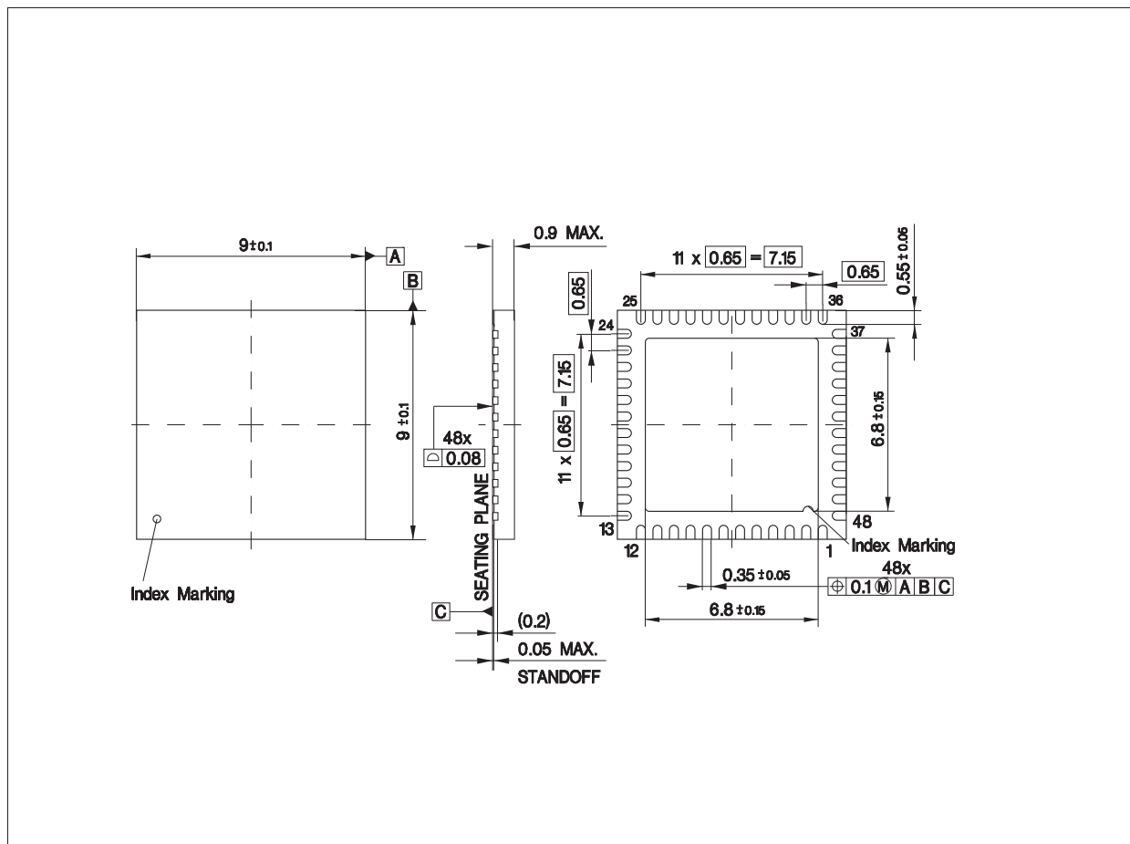
Figure 16 PG-VQFN-48
