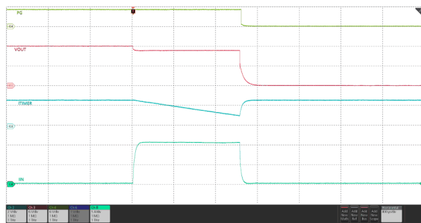
Figure 7-43. Circuit-Breaker Response TPS25974x
