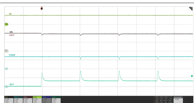
Figure 9-5. Transient Overload
