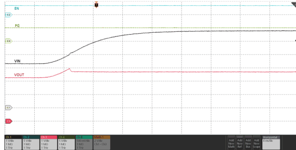
Figure 7-37. Overvoltage Clamp Response – TPS25972x
