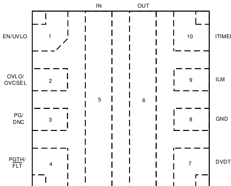
Figure 6-1. TPS2597xx RPW Package 10-Pin QFN (Top View)
