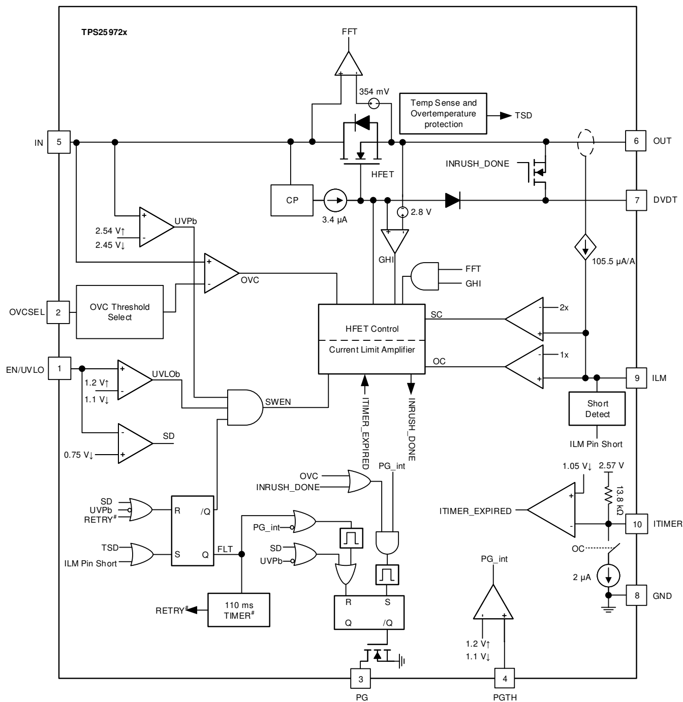
Figure 8-2. TPS25972x Block Diagram
