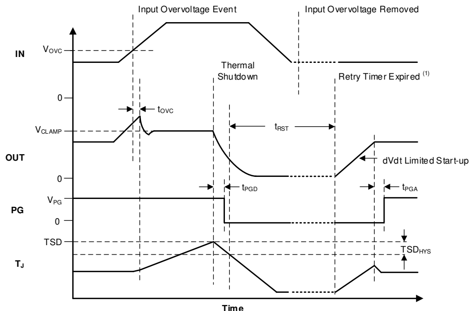
Figure 8-8. TPS25972x Overvoltage Response (Auto-Retry)
