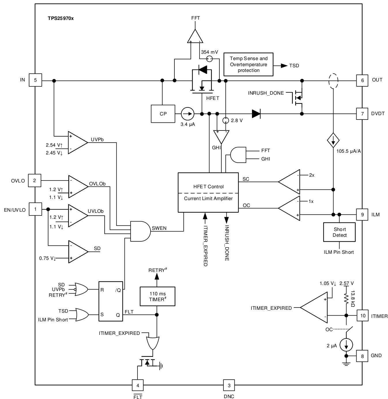
Figure 8-1. TPS25970x Block Diagram
