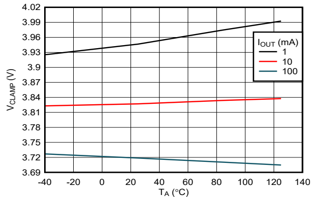
Figure 7-19. OVC Clamping Voltage (OVCSEL = GND) vs Load Current (TPS25972x Variant)
