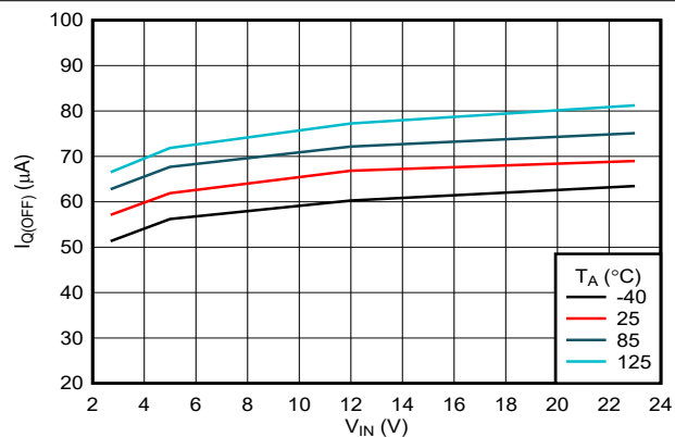
Figure 7-4. IN OFF State (UVLO) Current vs Temperature
