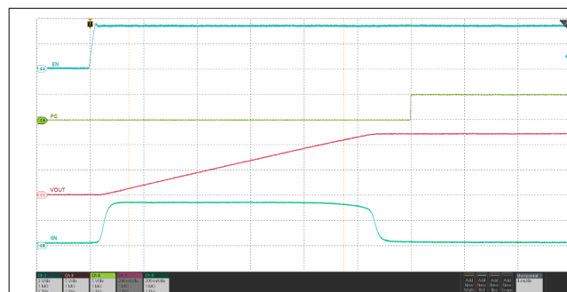
Figure 9-4. Power Up
