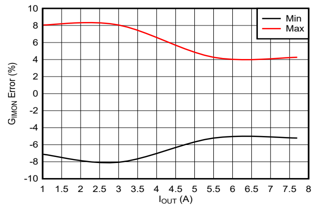
Figure 7-14. Analog Current Monitor Gain Accuracy
