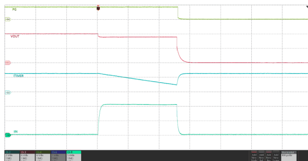
Figure 9-6. Circuit Breaker Response
