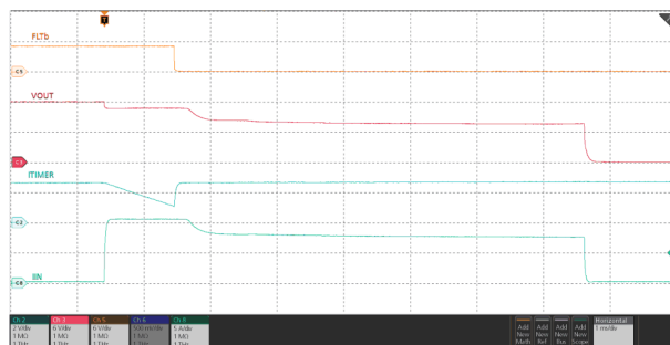
Figure 7-39. Overvoltage Clamp Response – TPS25972x
