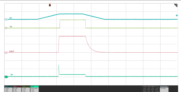
Figure 7-30. Power Up and Down With EN/UVLO Control V_{IN} = 12\text{ V} , C_{OUT} = 22\text{ }\mu\text{F} , C_{dV/dt} = \text{Open} , V_{EN/UVLO} ramped from 0\text{ V} \rightarrow 1.4\text{ V} \rightarrow 0\text{ V}
