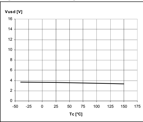
Figure 25. Undervoltage shutdown
