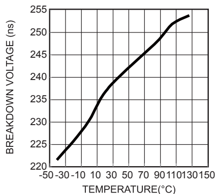
V D1,2 Breakdown Voltage vs. Temperature
