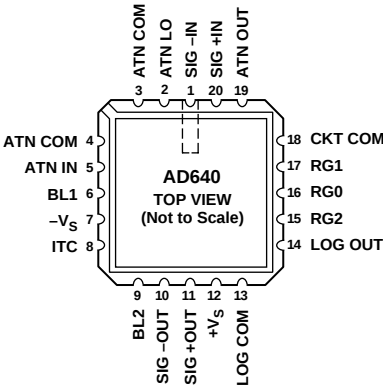
20-Terminal Ceramic LCC (E) Package
